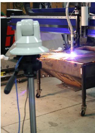
Remote Camera capturing live cutting.
